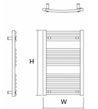
H80 – 14 tubes
