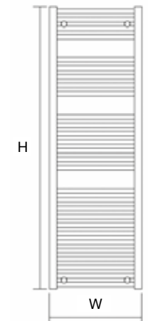
H150 – 28 tubes
