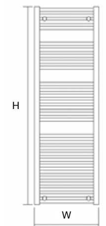
H150 – 28 tubes
