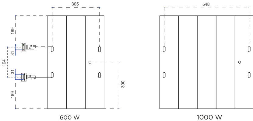
Fig. 3 - version 600 mm
