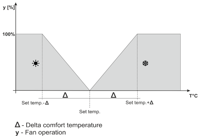
Figure 2. Chart of fan operation in the profile Comfort
