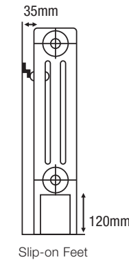
Slip-on Feet
